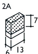
鑽石齒塊尺寸 The dimensions of diamond tips
